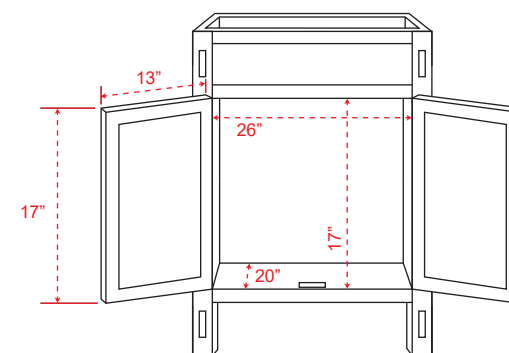
Front (open)
