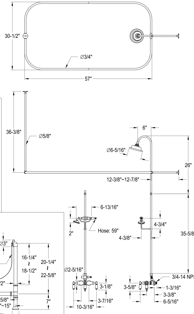
CC461,2,5,8 Single Offset Bath Supply
