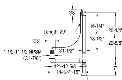
CC2091,2,5,8 Tub Waste & Overflow
