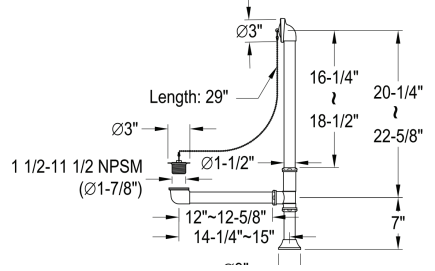
CC2091,2,5,8 Tub Waste & Overflow
