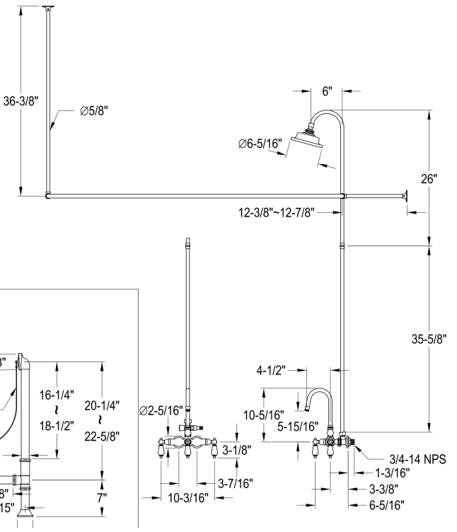
CC471,2,5,8 Double Offset Bath Supply
