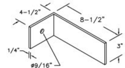
BRACKET DETAIL
