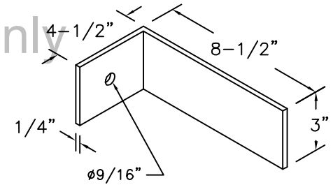
BRACKET DETAIL
