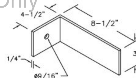
BRACKET DETAIL
